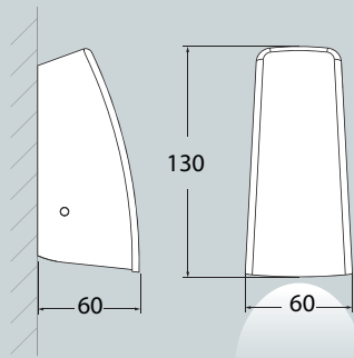
WALL INSTALLATION
