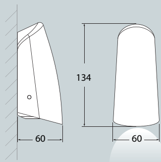
WALL INSTALLATION
